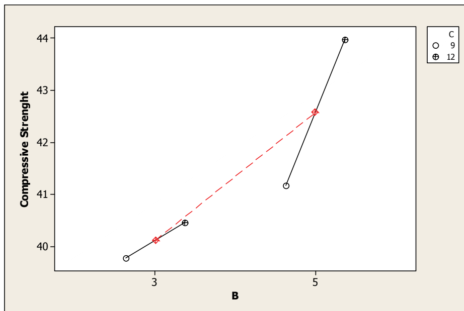
Figure 2. Multi-vari chart.
