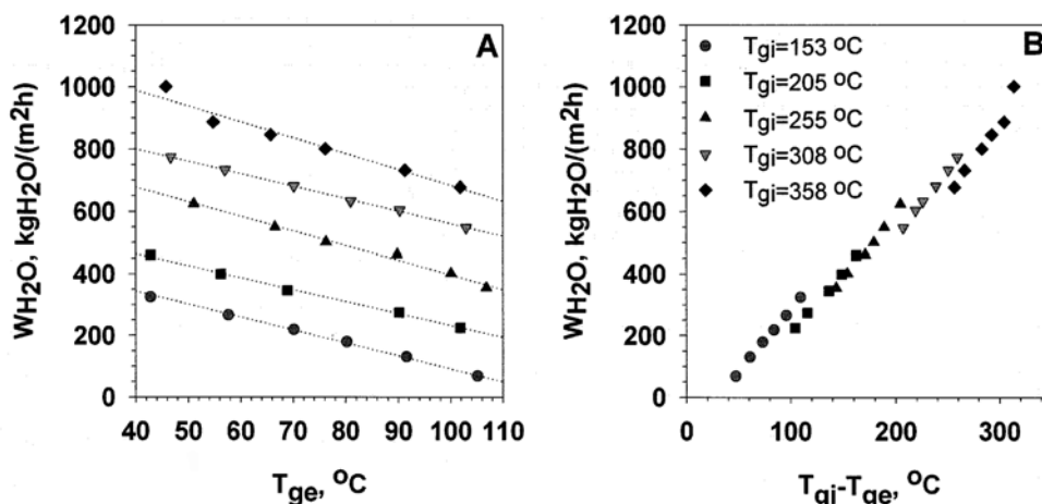
Slika 4. Specifična brzina isparavanja vode (doziranje tečne faze vode, U_0 = 1,77 m/s, inertne čestice, d_p = 1,94 mm) A – zavisnost od temperature sušenja, T_{ge} B – zavisnost od razlike temperatura, T_{gi} - T_{ge} Figure 4. Specific rate of water evaporation (feed – water, U_0 = 1,77 m/s, inert particles, d_p = 1,94 mm) A – function of drying temperature, T_{ge} B – function of temperature difference, T_{gi} - T_{ge}
