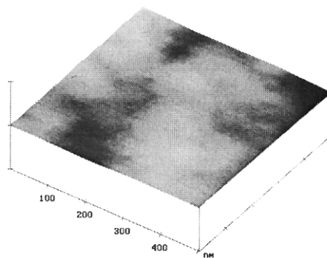
Slika 1. AFM slika polirane GC elektrode ( 500 \times 500 \times 100 nm) Figure 1. AFM images of GC (polished support) 500 \times 500 \times 100 nm
