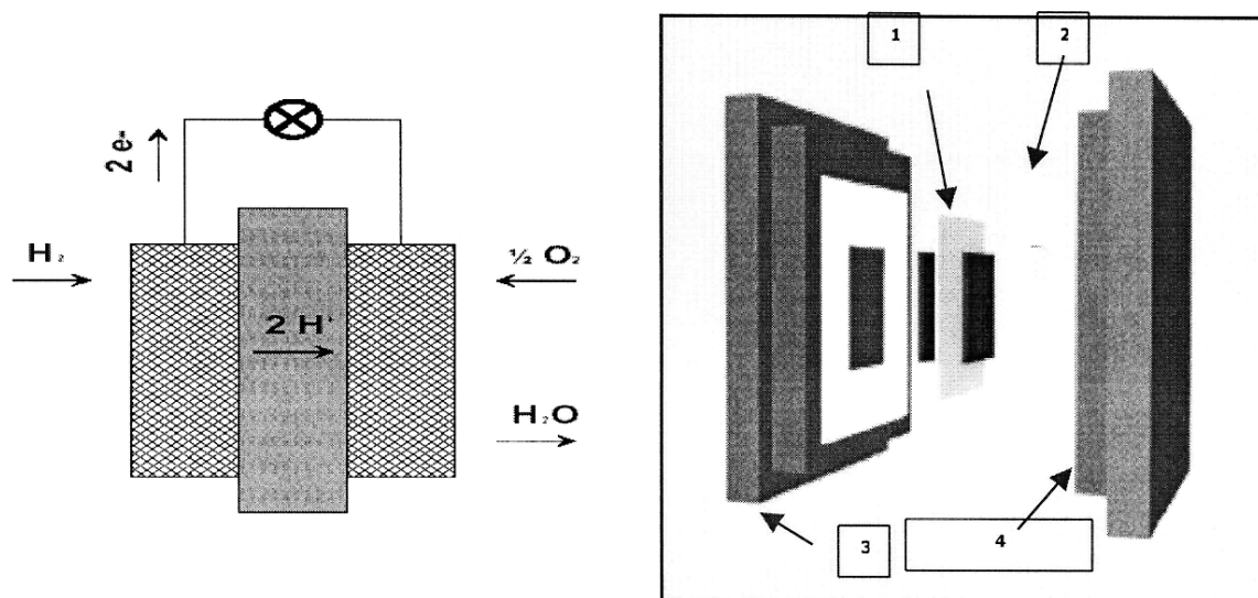
Figure 1. Principle of H_2/O_2 Polymer Electrolyte Fuel Cell reactions and single cell components
