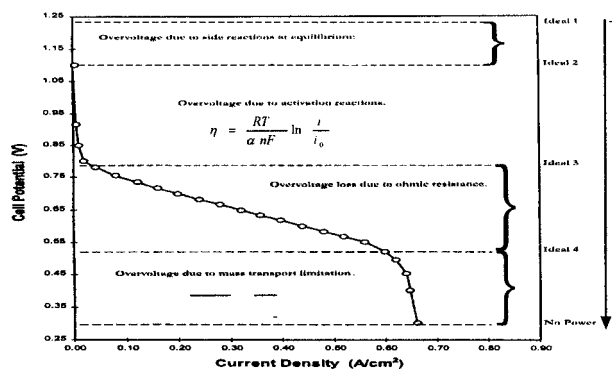
Figure 4. Various contributions of potential loss: The loss of potential related to cathode lack of activity is from ideal 1 to ideal 3, e.g. at least 60% of the cell potential.
