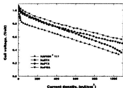
Figure 2. [7,12] Potential-current polarisation curves of H_2/O_2 fuel cells using Nafion ® 117 (thickness = 180 \mu m and water uptake of 30%), NaSTA (thickness = 175 \mu m and water uptake of 60%), NaPTA (thickness = 165 \mu m and water uptake of 70%) and NaPMA (thickness = 160 \mu m and water uptake of 95%).
