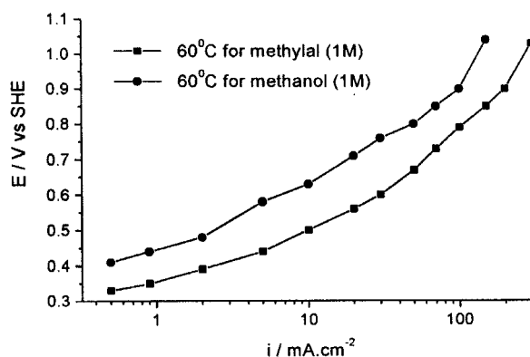
Figure 6. Quasi-steady-state polarisation curves for the direct electro-oxidation of methylal (60°C) and methanol (60°C) in 1 M H 2 SO 4 .
