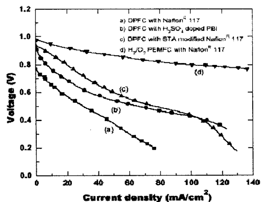
Figure 10. V-I curves of Direct propane/oxygen PEFC
