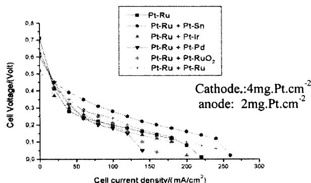
Figure 9. V-I curves of Direct Acetal/ O_2 PEFC
