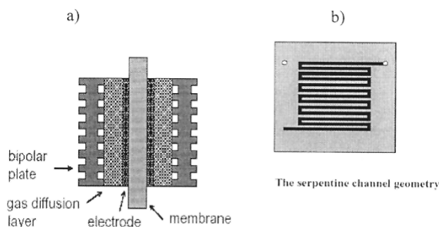
Figure 5. PEFC simple diagram [30] a) Structure with bipolar plates; b) The most type of channel used in bipolar plates design
