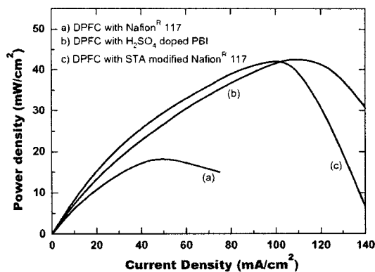
Figure 11. Power density vs current density plots derived from Fig. 10
