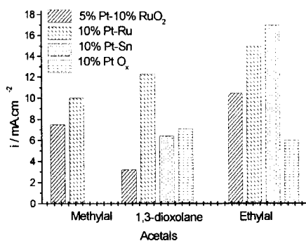
Figure 7. Bar chart representation of direct electro-oxidation current density for methylal, 1,3-dioxolane and ethylal in 1 M H_2SO_4 at 25°C and 0.6 Volt vs SHE on various electrode materials
