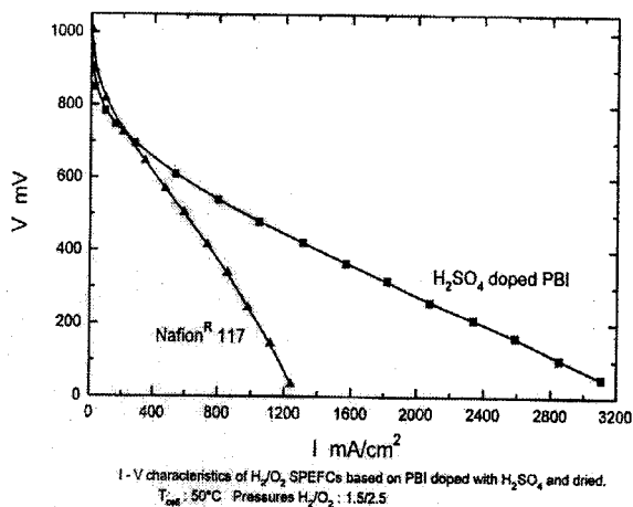
Figure 3. V-I curves of H_2/O_2 PEFC [13]
