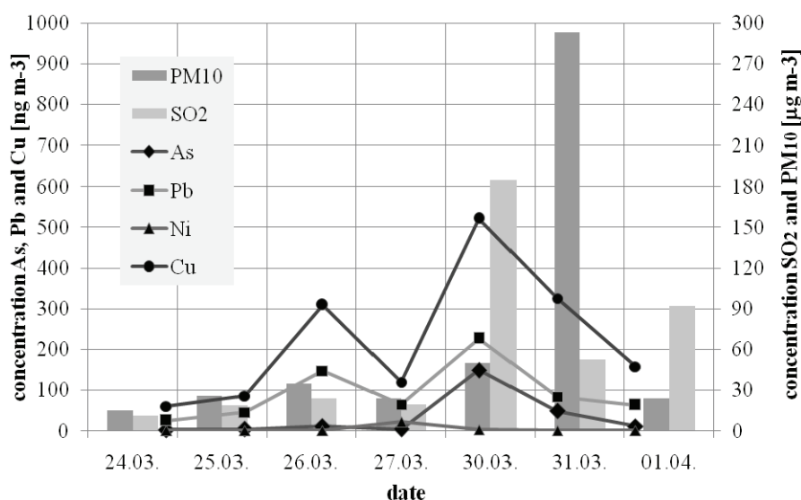
Figure 2. Daily average values of selected metals concentration in PM 10 , and PM 10 and SO 2 concentrations during sampling campaign, spring 2009.
