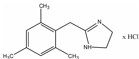
Figure 1. Chemical structure of trimazolin hydrochloride.
