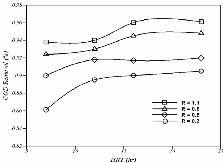
Figure 4. The effect of HRT on COD removal for various sludge recycle ratios at averaged COD , 27 \text{ }^\circ\text{C} , 30 \text{ l} aerated vessel.
