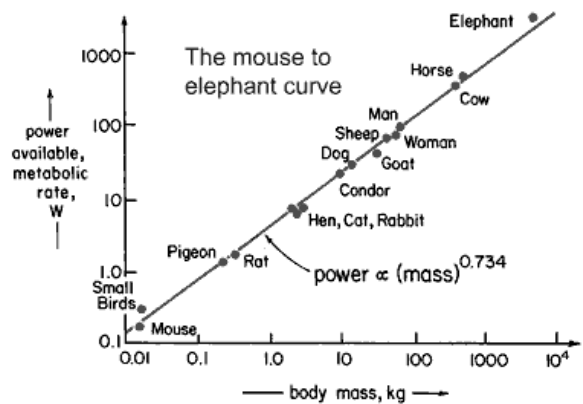
Figure 4. The "mouse-to-elephant" curve shows that the power of a warm blooded animal is proportional to its mass to the 0.734 power, as given by eq. 1.
