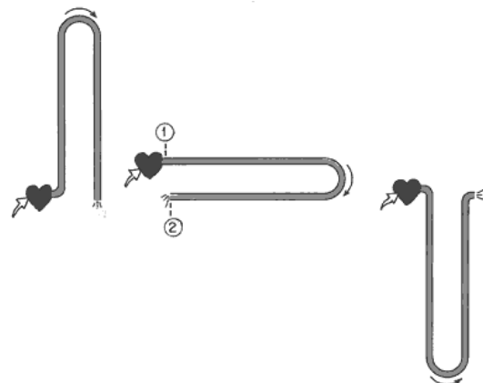
Figure 11. From the first law of thermodynamics the three flow systems in this figure all require the same pumping power
