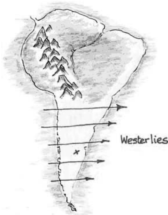
Figure 3. Southern South America minus the Andes mountain range will allow strong prevailing westerly winds to blow continually
