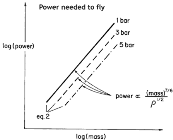
Figure 5. Aeronautics plus thermodynamics tells that the power needed to stay aloft depends on the creatures mass and the atmospheric density, as given by eq. 2.
