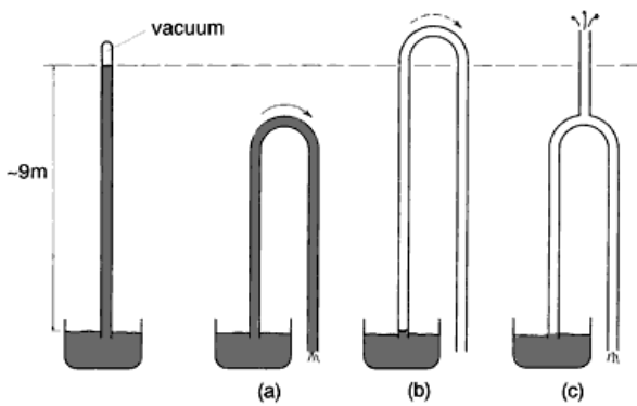
Figure 12. (a) Water siphons less than about 9 m high will work [20]. (b) Above about 9 m will not work. (c) Partial siphons have been proposed [16] but are just nonsense.
