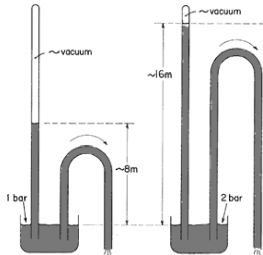
Figure 14. With a higher atmospheric pressure taller siphons will work
